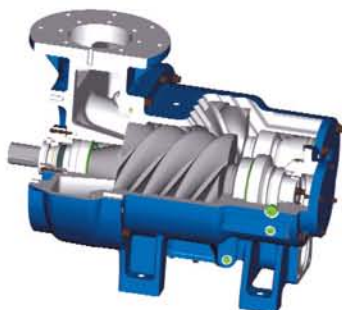
Rotary Screw Gas Compression Module
