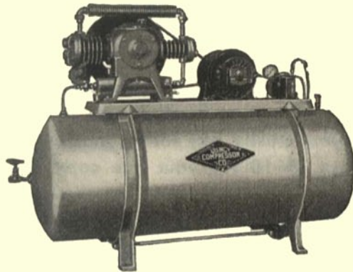
Model G-18. Two-Stage Air Cooled Automatic Unit. Vee Belt drive. Tank, 20 x 48—65 gals. 175-lb. cut-off pressure. Displacement, 3 3/4 ft. with 3/4 H.P. motor; 4 1/2 cu. ft. with 1 H.P. motor; 6 cu. ft. with 1 1/2 H.P. motor; 7 1/2 cu. ft. with 2 H.P. motor. Equipment includes 25-ft. hose with chuck, compressor muffler, outlet valve and all fittings.
